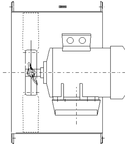
Spalt "s" in mm bei Ex-Ventilatoren/ gap "s" in mm for ex-fans
